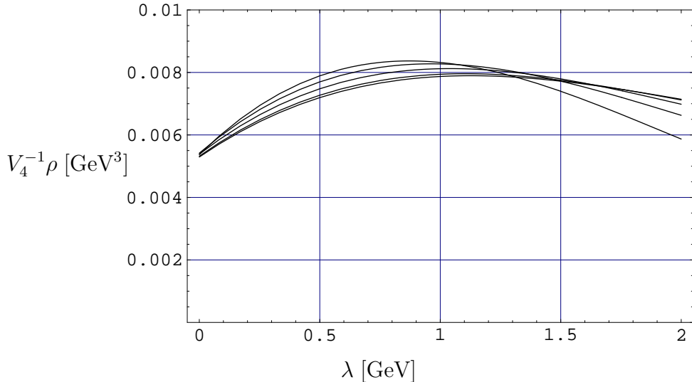
Figure 6: The spectral density for different regulator functions f_k^{(n)} . The uppermost curve corresponds to n=2 . The others are respectively n = 3, 5, 10, 15 , where the last two are already nearly equal.
